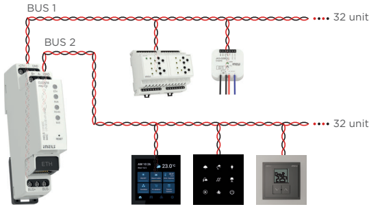
Central unit
