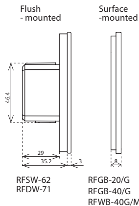
Flush - mounted
