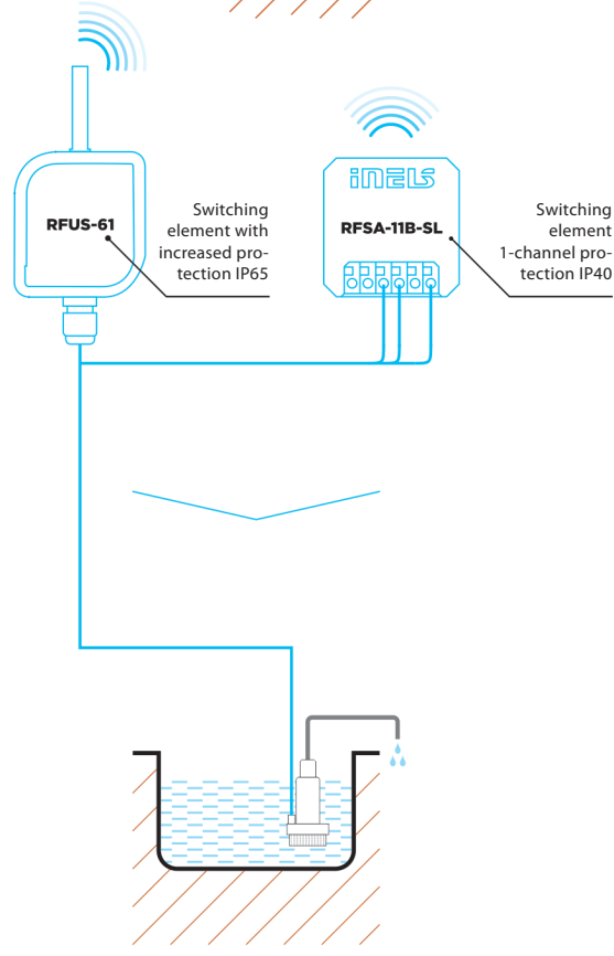
Control of 1 pump: RFS-11B-SL, RFUS-61 Control of 2 pumps: RFS-62B-SL
