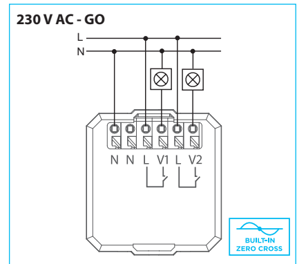
The output contacts (V1, V2) are galvanically isolated from the power supply and each has its own COM terminal. However, they must be connected to the same phase
