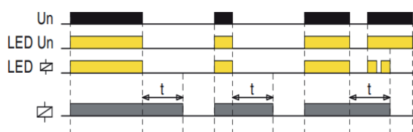
a True OFF Delay
